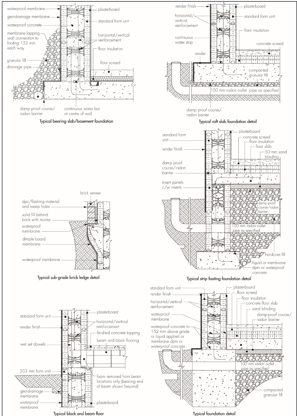
Figure A3 Typical construction details
